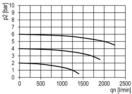
flow characteristic
